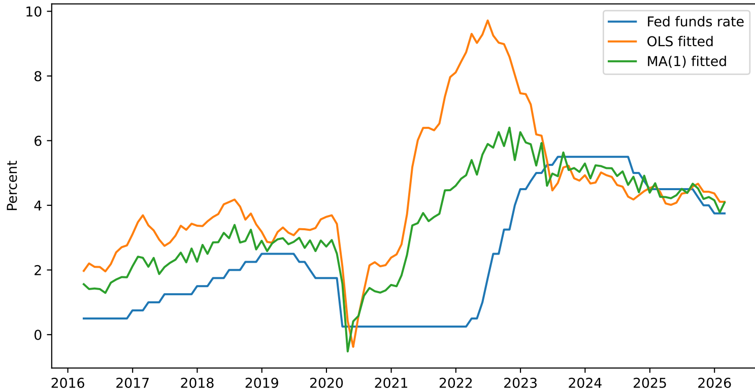
Dataset 1 - Taylor rule fitted values (last 120 observations)
